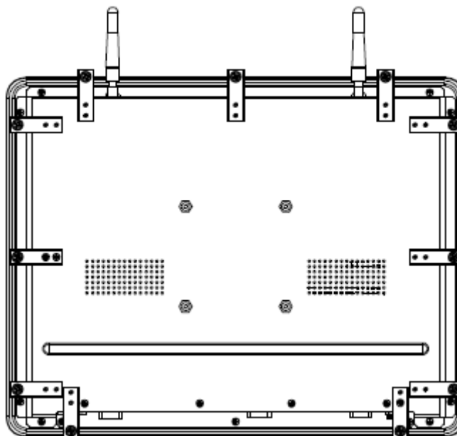
Figure 10 Panel Mounting
