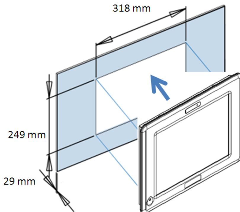
Figure 9 Panel Mount Cut-out hole and maximum panel thickness
